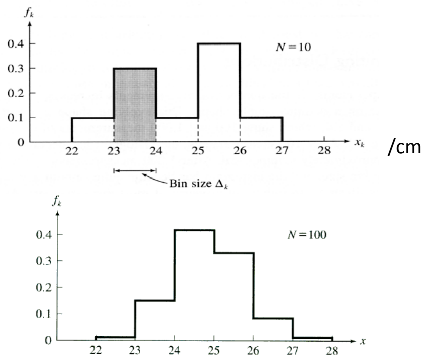
Figure 5.3. Histogram for 100 measurements of the same quantity as in Figure 5.2.
