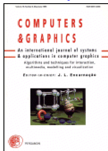
Computers & Graphics
