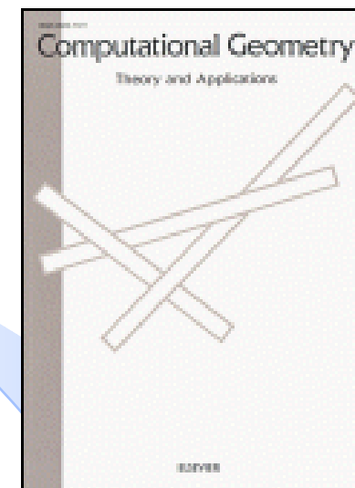
Computational Geometry
