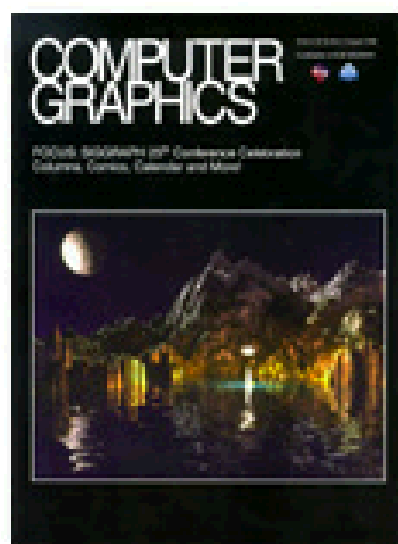
Computer Graphics
