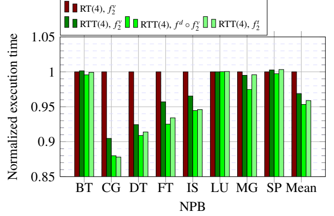
Figure 11. Execution time for 64 processes mapped onto a RT(4) or RTT(4) with c = 2
